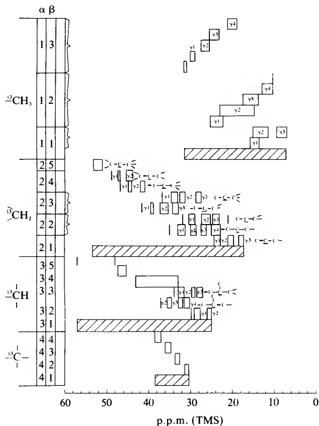
Fig. 3.49 Graphical display of chemical shifts for classes of paraffins. Data reproduced from L. P. Lindemann and J. Q. Adams (1971). Analyt. Chem. , 43(10), 1251.
