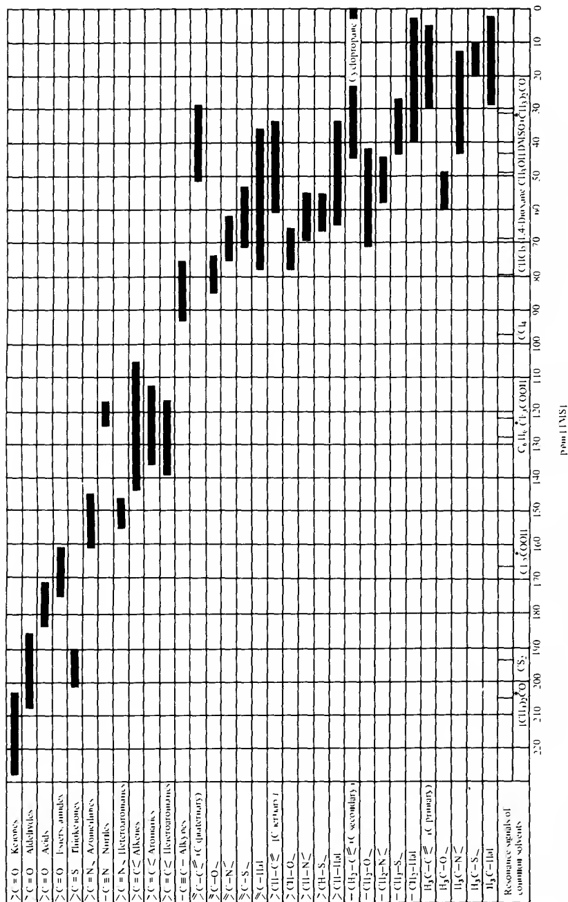
Fig. 3.45 ^{13}\text{C} chemical shifts in organic compounds. Data reproduced from E. Breitmaier, G. Jung and W. Voelter (1971). Angew. Chem. Int. Edn. Engl. , 10, 679.
