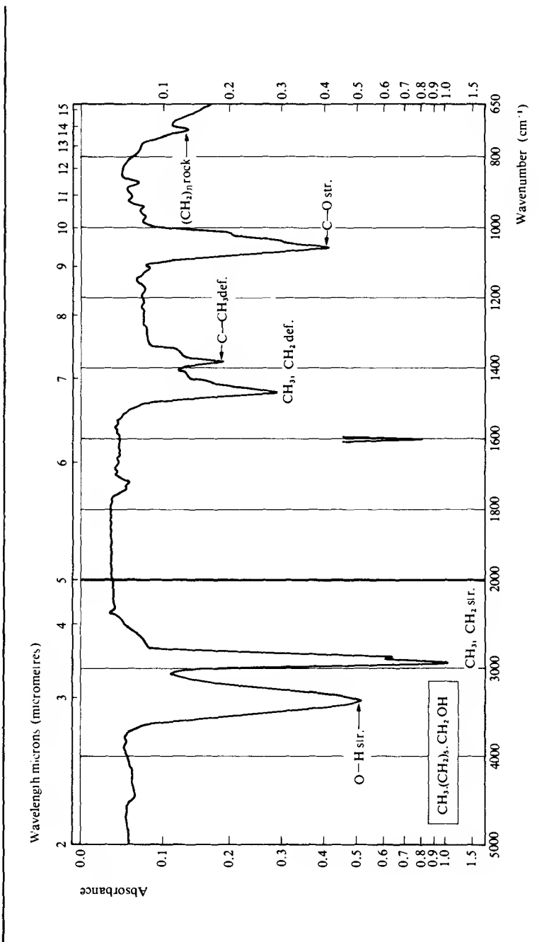
Fig. 3.21 Infrared spectrum of heptan-1-ol recorded as a liquid film.
