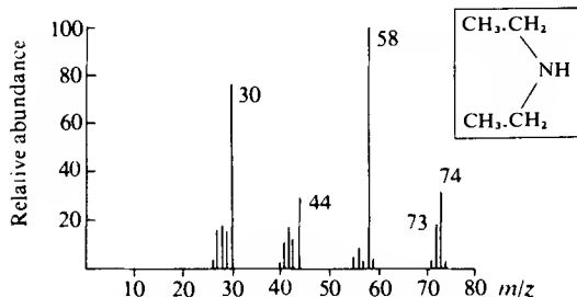
Fig. 3.87 Mass spectrum of diethylamine.
