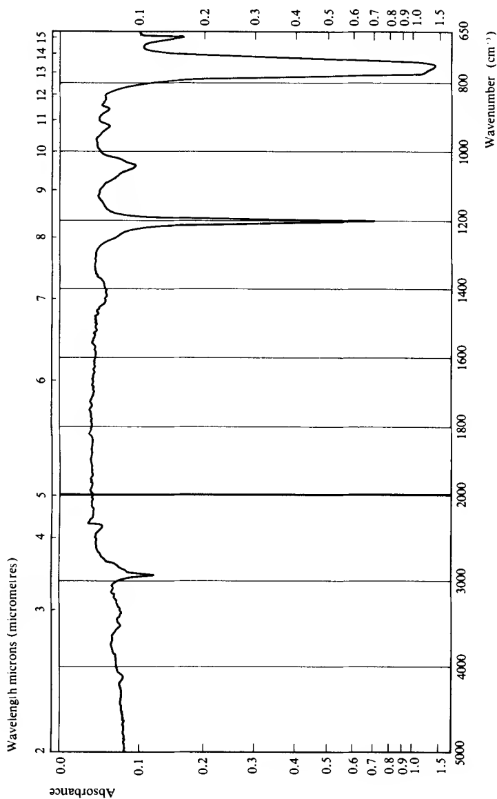
Fig. 3.5(a) Chloroform.
